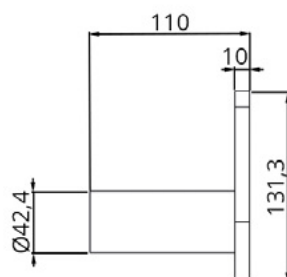
104283 Flat bracket mounting arm 110 mm. Bottom plate thickness 10 mm.
