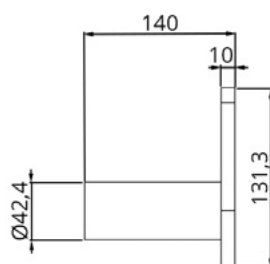
104285 Flat bracket mounting arm 140 mm. Bottom plate thickness 10 mm.
