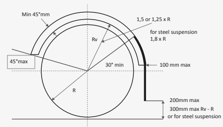
Absorber for one axle
